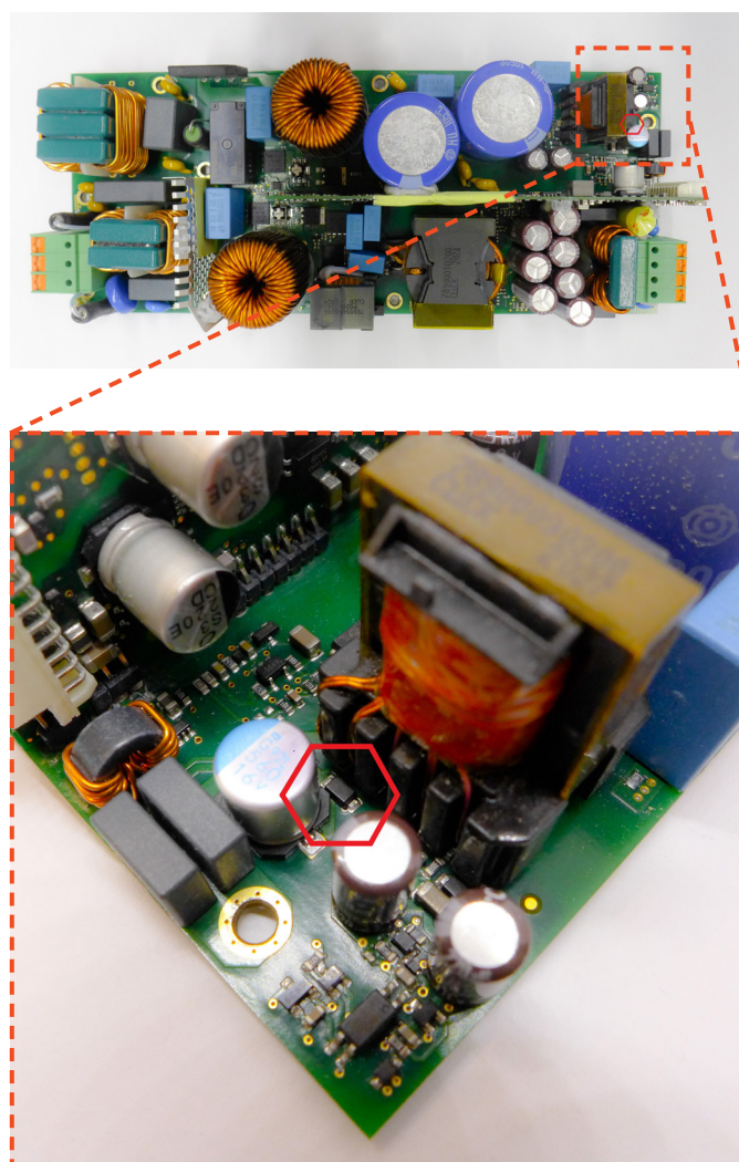
Figure 3: High density PCB of RACM1200-V including PMEG100T20ELR
