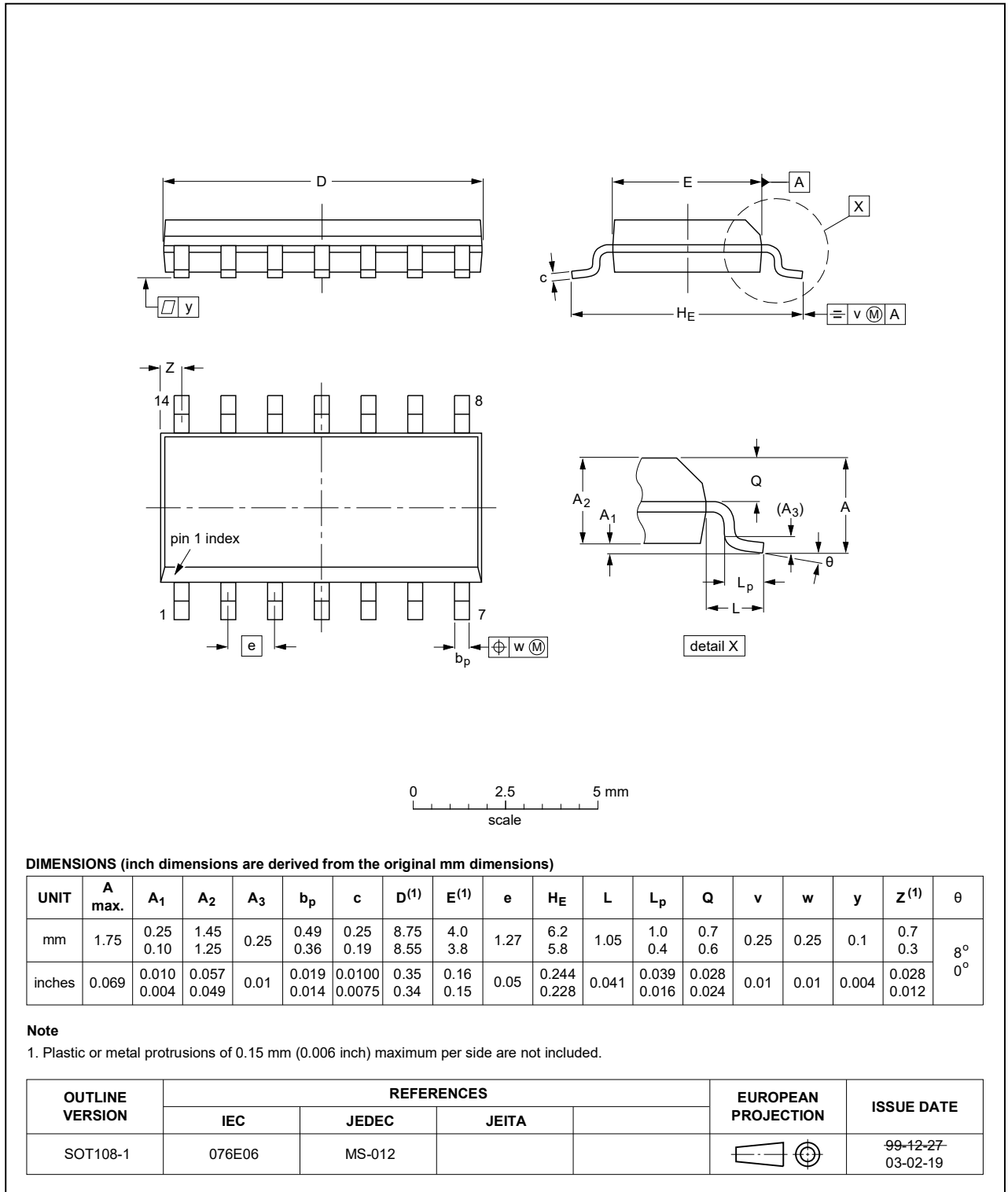
Fig. 1. Package outline SO14 (SOT108-1)
