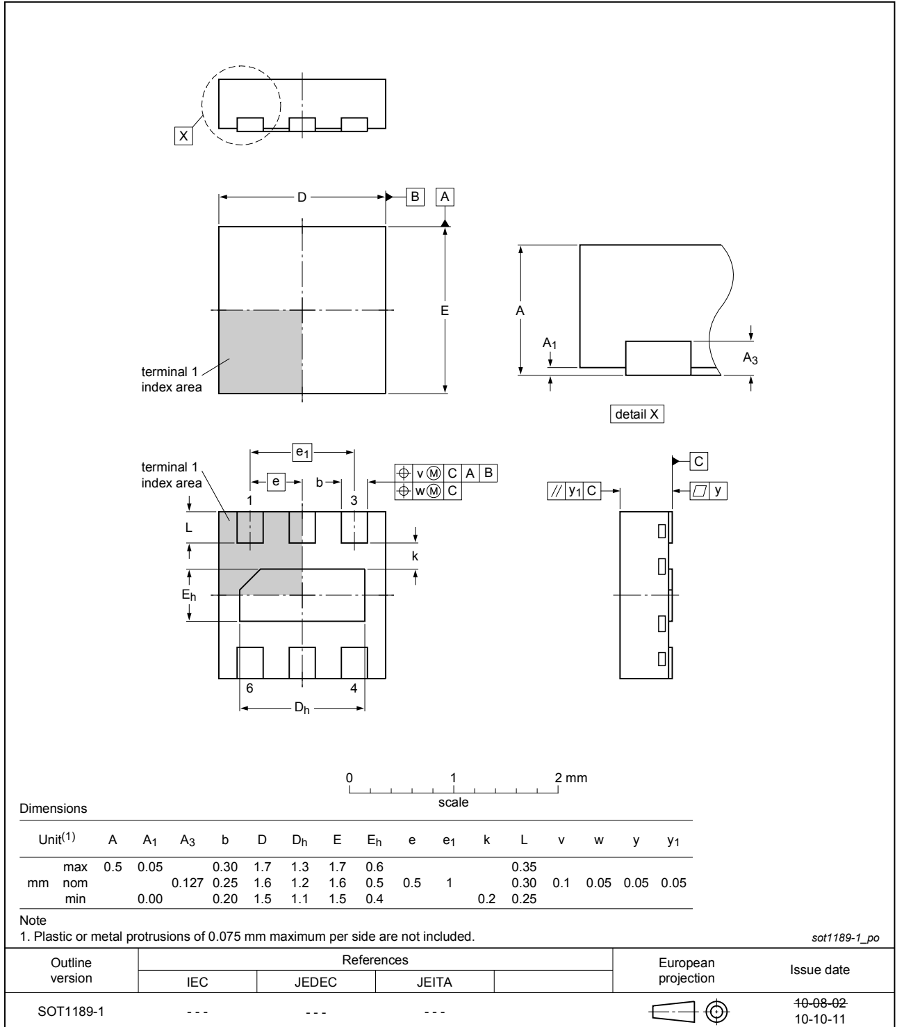
Fig. 1. Package outline DFN1616-6 (SOT1189-1)
