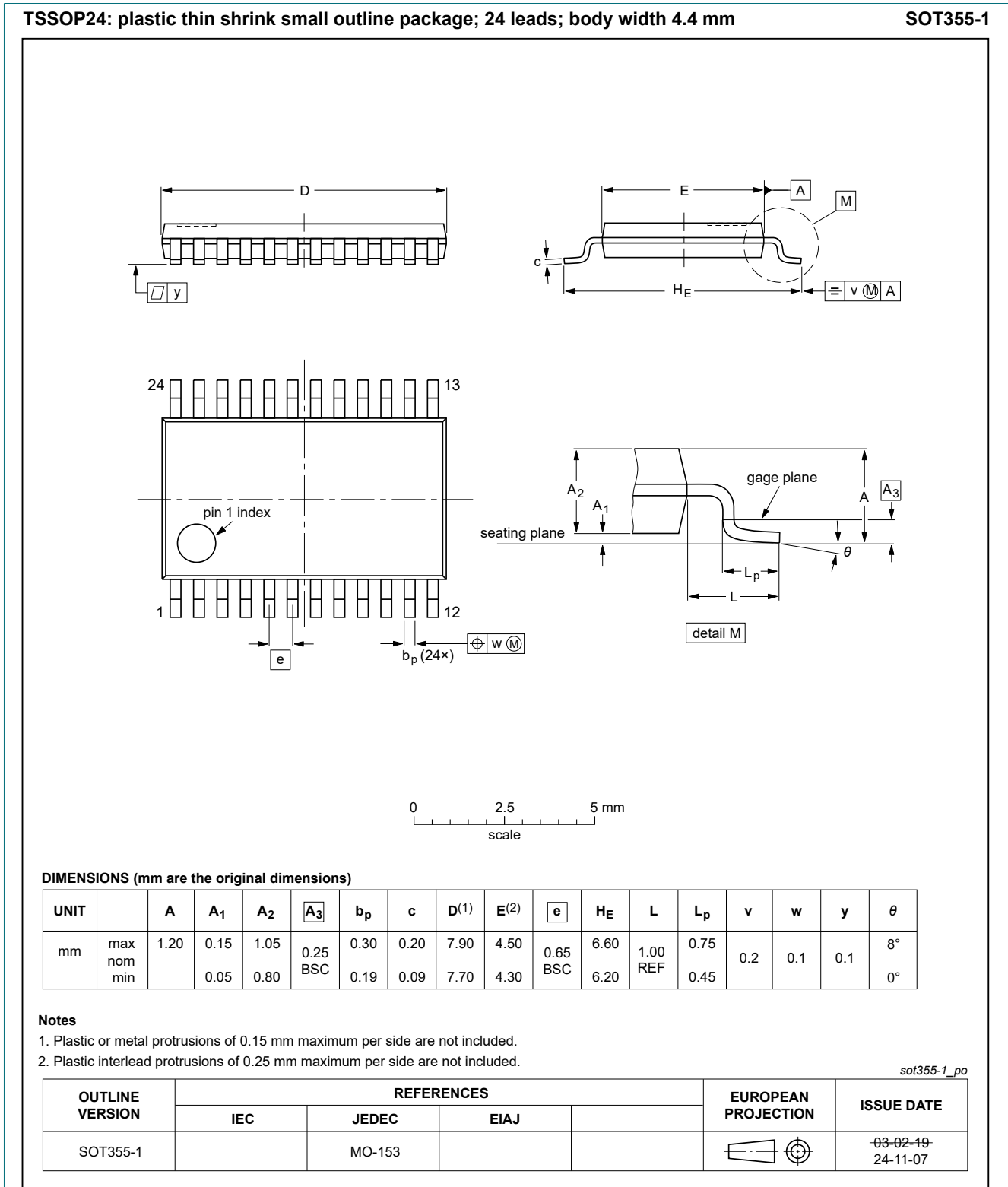
Fig. 1. Package outline TSSOP24 (SOT355-1)
