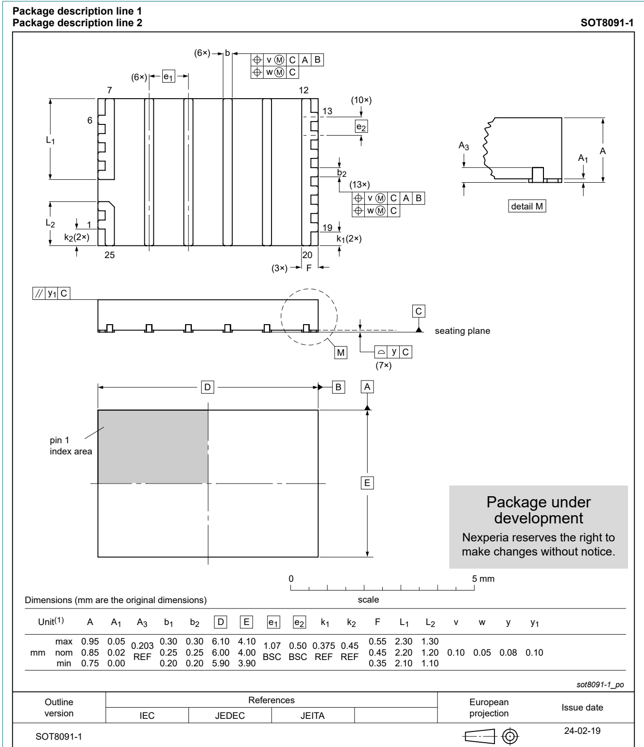
Fig. 1. Package outline VQFN7 (SOT8091-1)
